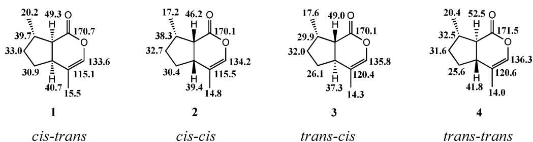
Figure 3. Unambiguously assigned ^{13}\text{C} NMR shifts of all nepetalactones.
