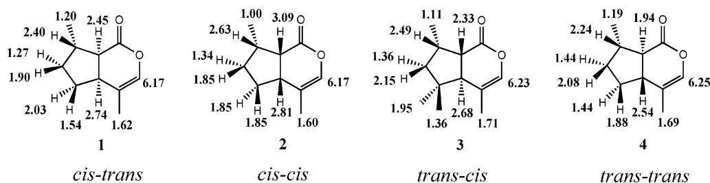
Figure 4. ^1\text{H} NMR shifts of all nepetalactones.
